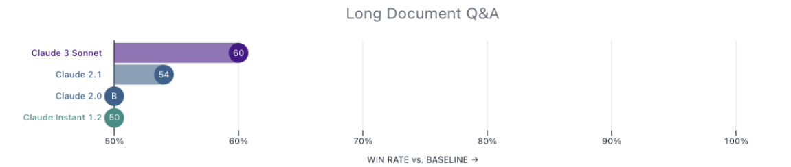
Figure 5 This plot shows per-task human preference win rates against a baseline Claude Instant model for common use cases.
