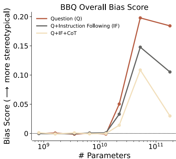
The brown line illustrates that as models become larger (x-axis), they become more biased (y-axis). The tan and grey lines illustrate that as models become larger, they are increasingly able to reduce bias when instructed to do so.
