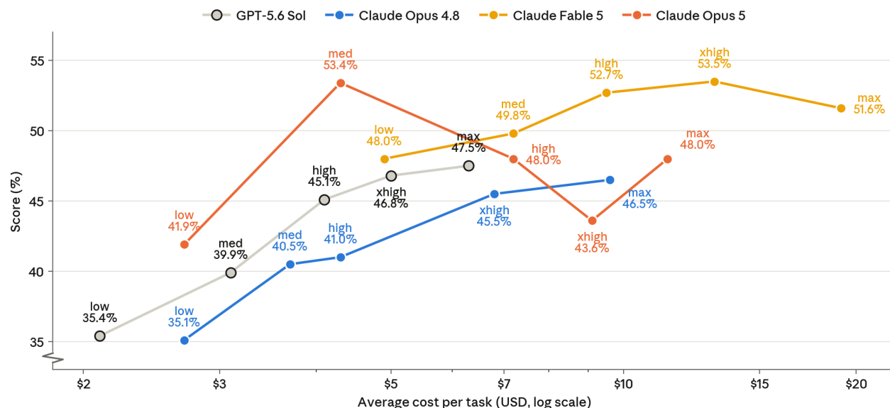
[Figure 8.4.A] FrontierCode (main set). Scores of Claude Opus 5, Claude Opus 4.8, Claude Fable 5, and GPT-5.6 Sol on the main set of FrontierCode v1.1, a coding evaluation run and scored by Cognition, at each model's five reasoning-effort settings. Claude Opus 5 reaches its best main-set score, 53.4, at medium effort.
