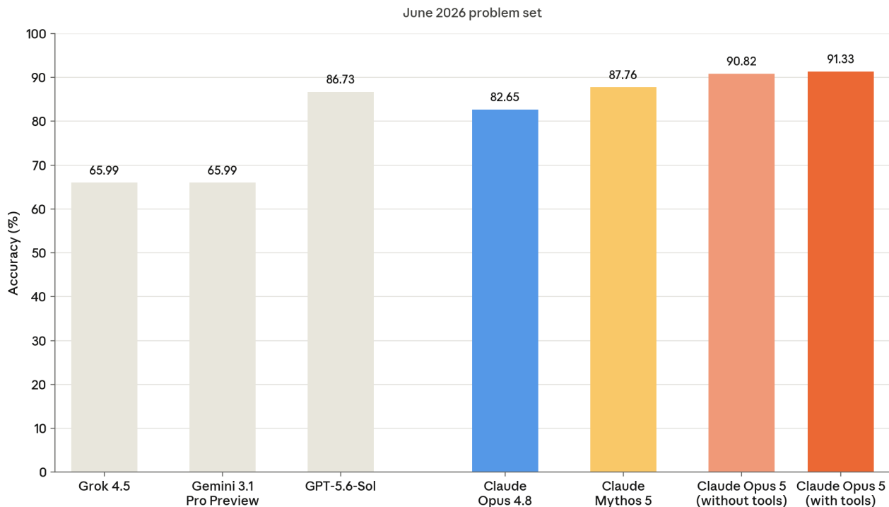
[Figure 8.8.A] ArxivMath (June 2026) accuracy scores. Claude Opus 5, Claude Mythos 5, and Claude Opus 4.8 were evaluated internally with max effort; other scores are from the MathArena leaderboard. 16 Except for Claude Opus 5 (with tools), other scores are without access to tools.
