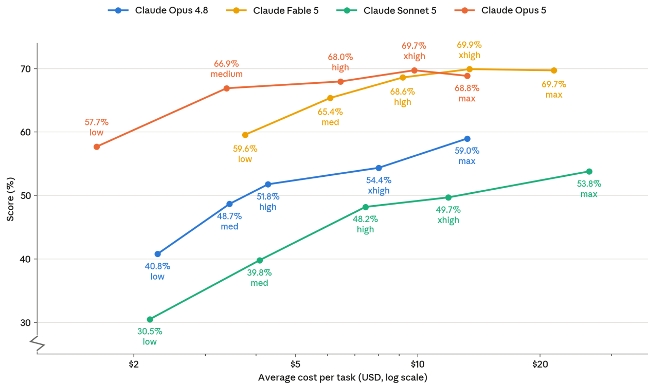
[Figure 8.3.A] DeepSWE v1.1 score versus average cost per task across reasoning-effort levels.
