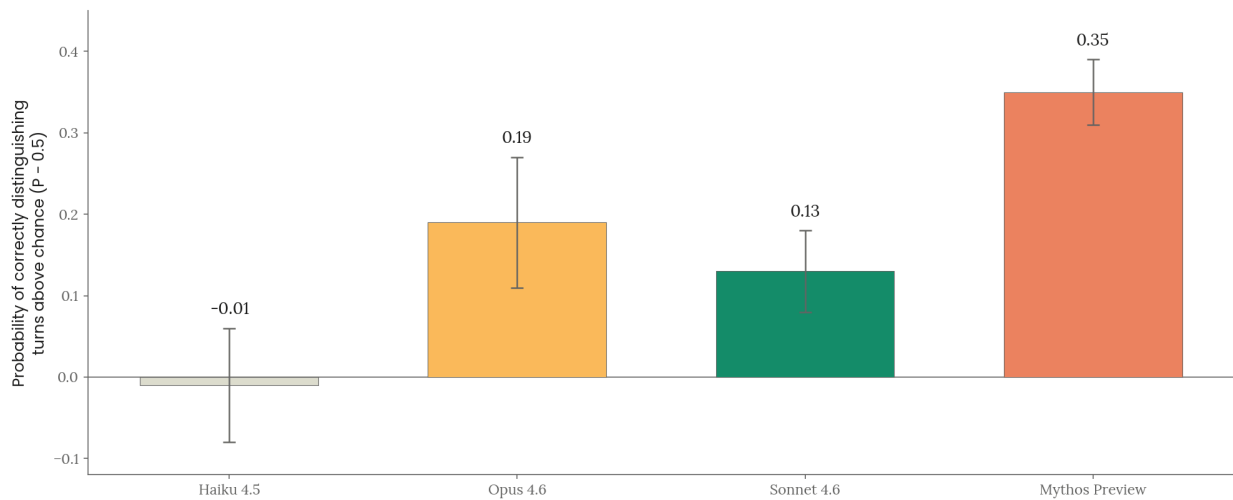
[Figure 77.A] Accuracy at distinguishing real from model-generated user turns. Each model serves as both generator (writing synthetic user messages) and judge (telling real from synthetic) on paired Claude Code transcripts.
