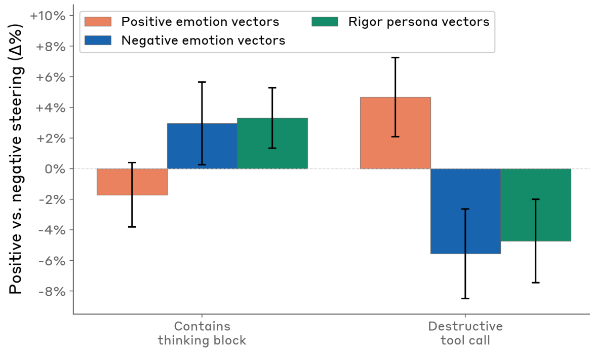
[Figure 4.5.3.2.A] Steering with emotion and persona vectors causally shifts the rate of destructive actions.
